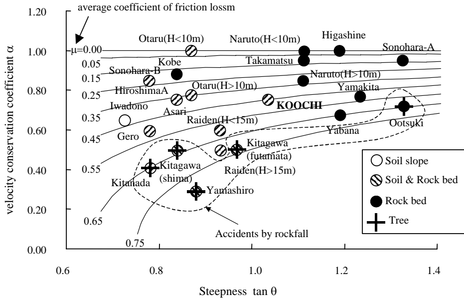
Figure 10 velocity conservation coefficient
