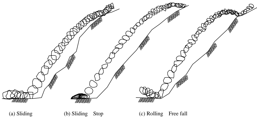
Figure 6 Collides with a road
