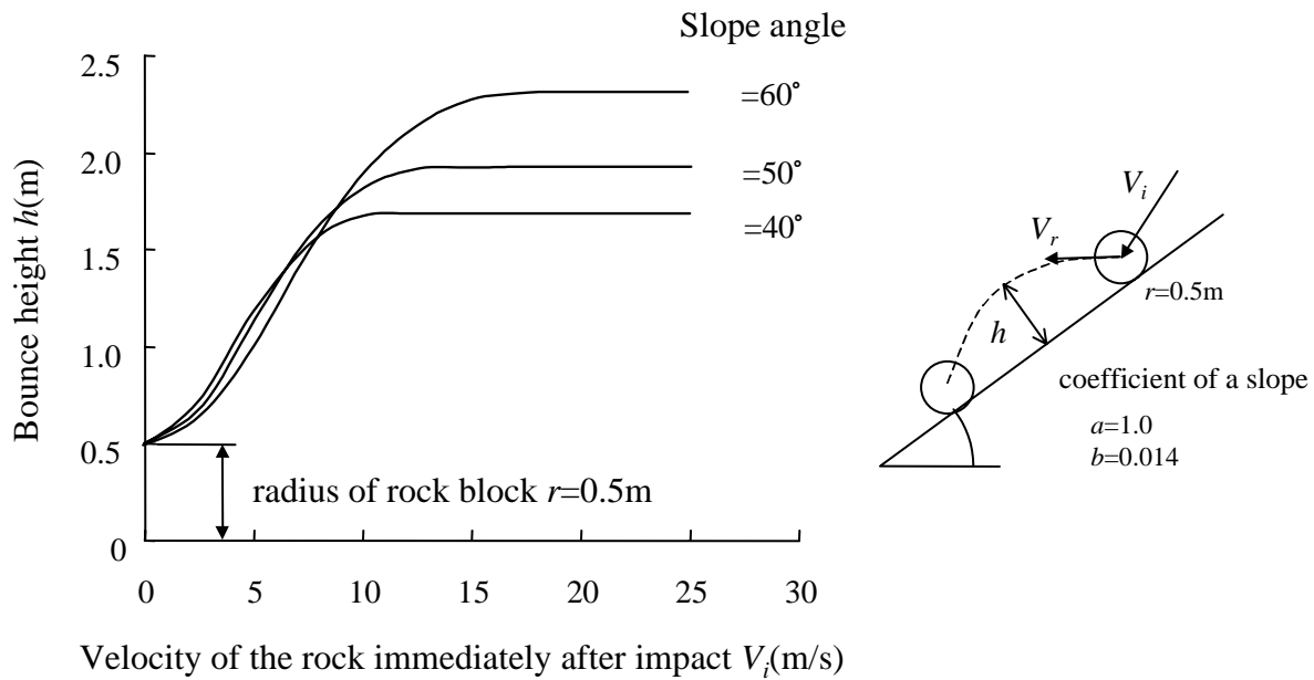
Figure 14 Bounce height as per the calculation
