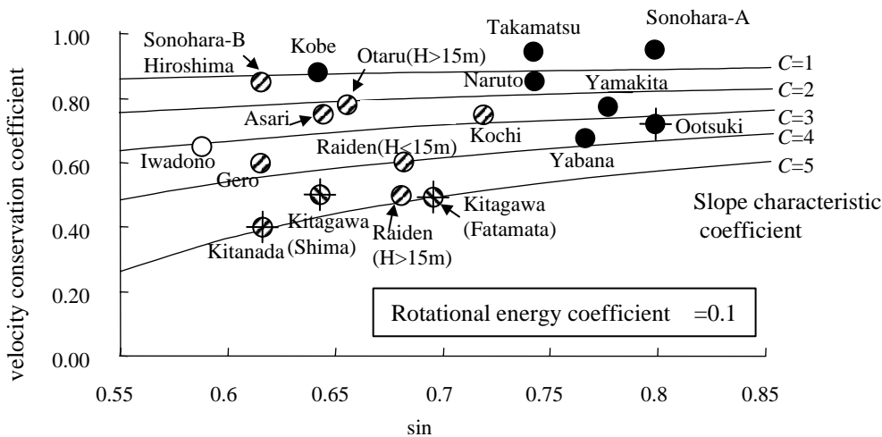
Figure 13 velocity conservation coefficient
