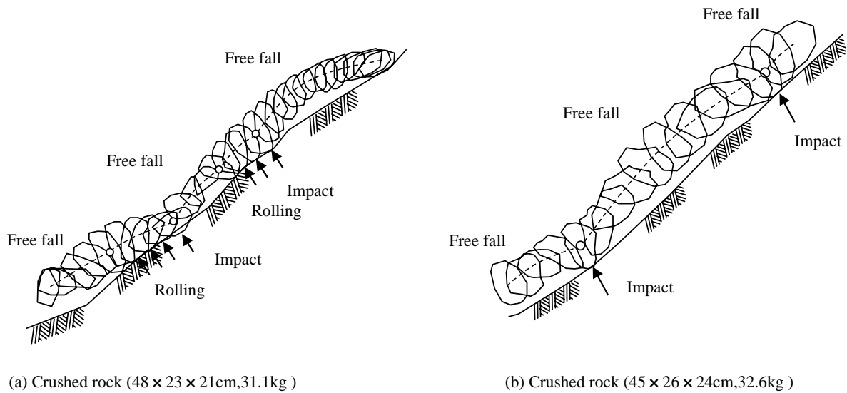
Figure 5 Impact and bouncing
