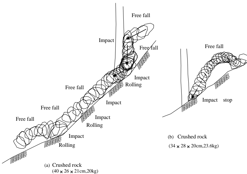
Figure 7 Collides with a tree
