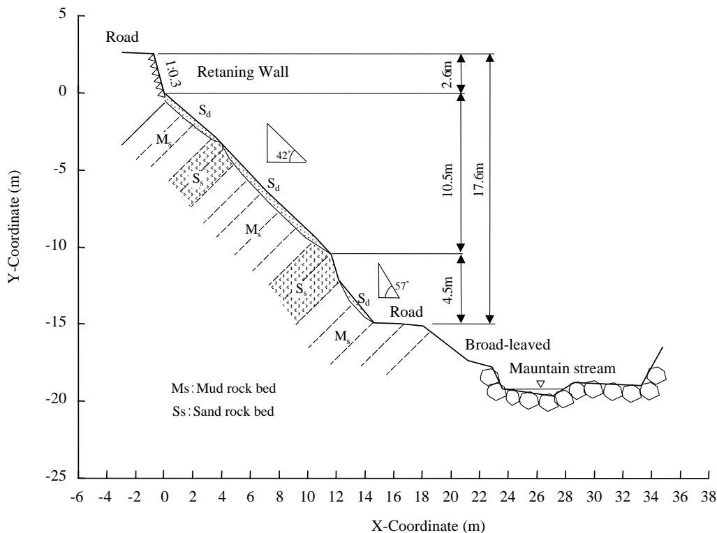
Figure 2. profile of the experimental slope
